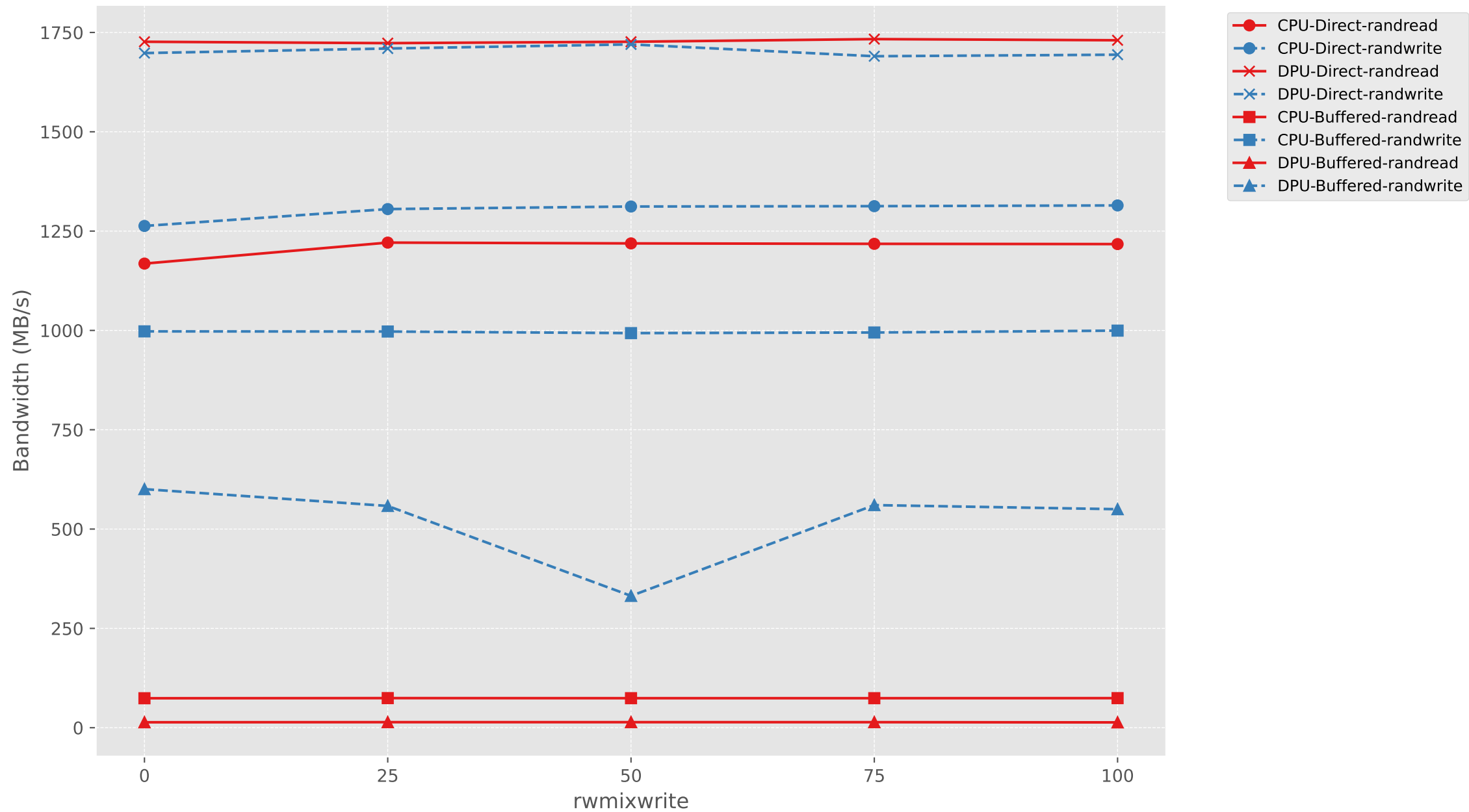
Bandwidth vs rwmixwrite (CPU vs DPU, Direct vs Buffered)
